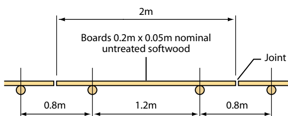
Figure 4.1.2 PLAN OF TOE BOARDS
